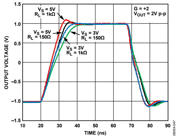
Figure 35. Large-Signal Step Response, G = +2
