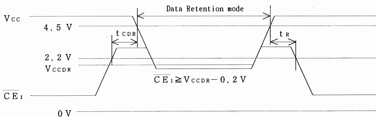
Data Retention timing chart - ( \overline{CE_1} Controlled) (*16)
