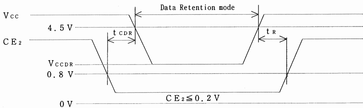
Data Retention timing chart - ( CE_2 Controlled)
