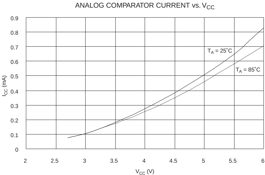
Figure 77. Analog Comparator Current vs. V_{CC}
