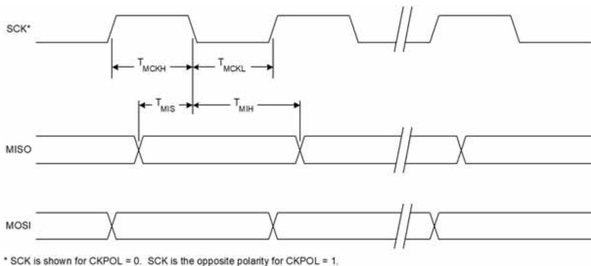
Figure 16.7. SPI Master Timing (CKPHA = 1)
