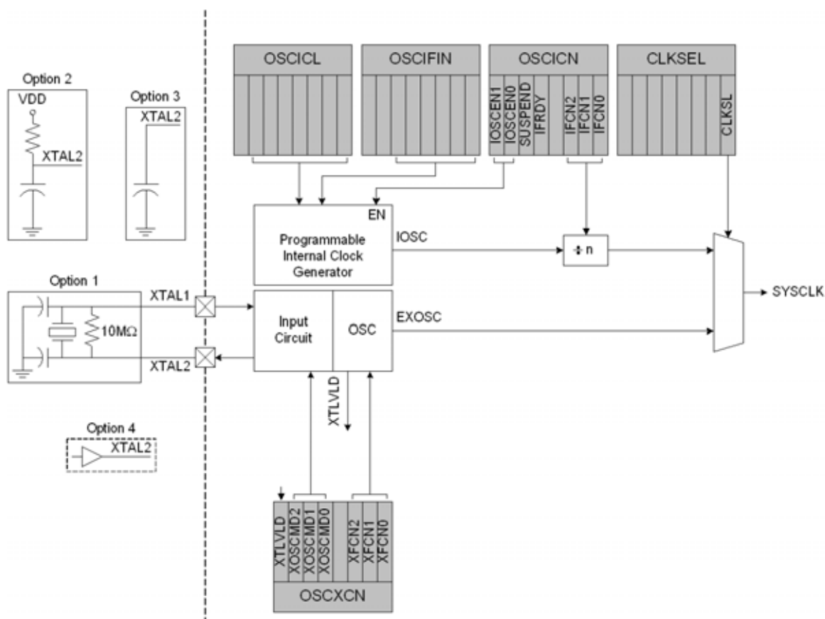
Figure 14.1. Oscillator Diagram
