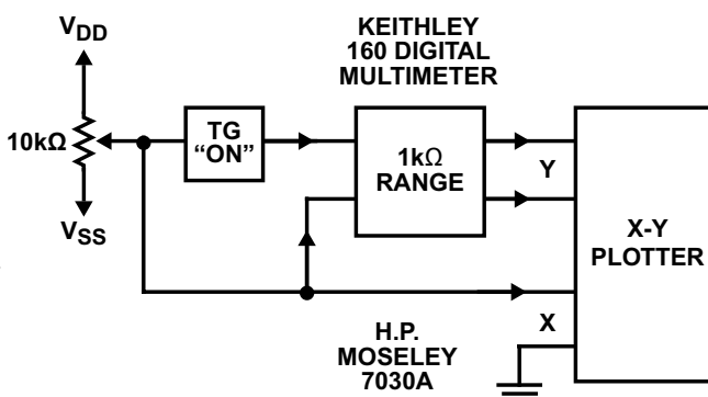
Figure 7-11. Channel ON Resistance Measurement Circuit
