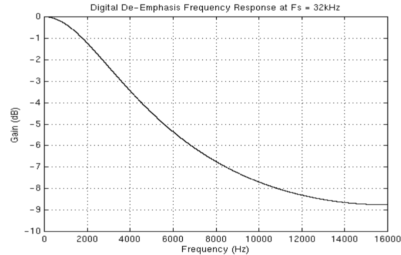
Figure 42. De-Emphasis Filter Response at 32 Ksps
