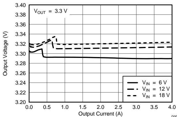
Figure 4. VO1=3.3\text{V} Output Voltage vs Output Current
