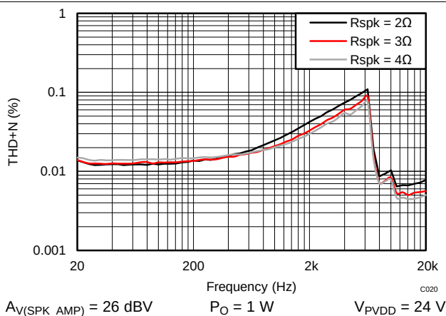
Figure 46. THD+N vs Frequency – PBTL
