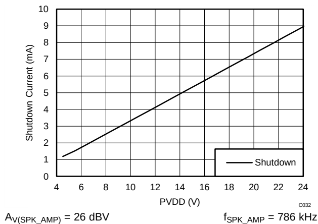
Figure 59. Powerdown Current Draw vs PVDD – PBTl
