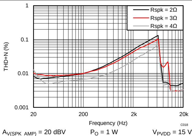
Figure 44. THD+N vs Frequency – PBTL
