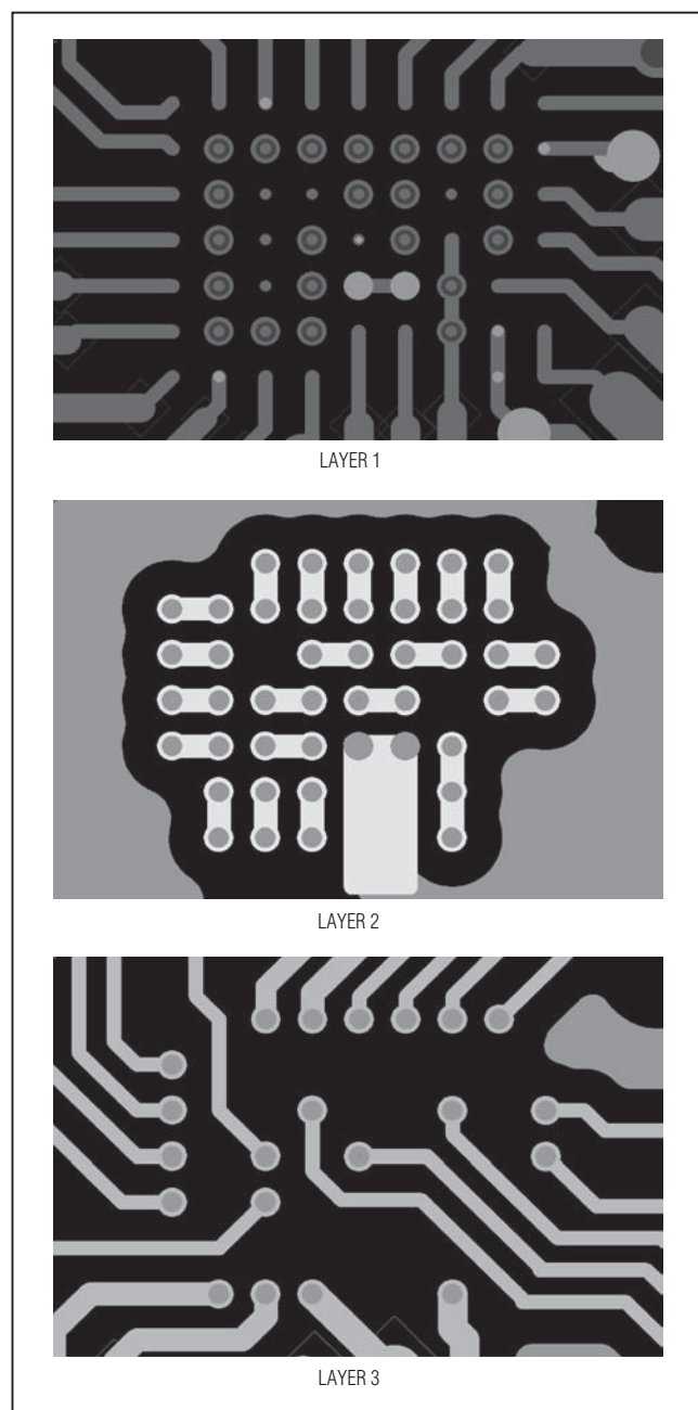
Figure 42. Suggested Routing
