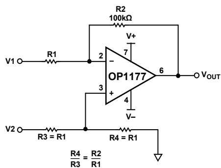
Figure 63. Difference Amplifier
