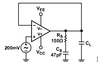
Figure 43. Snubber Network
