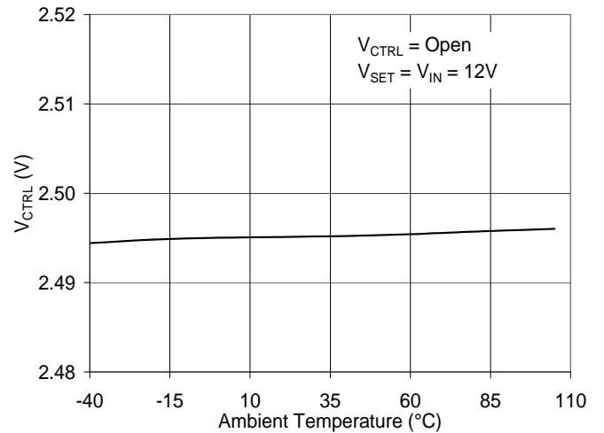
Figure 4 V_{CTRL} vs. Temperature
