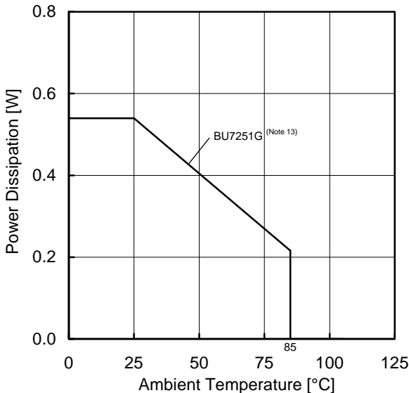
(c) BU7251G
