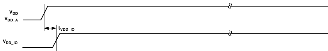
Figure 12. Power-Up Timing
