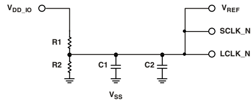
R1: 2kV SERIES RESISTOR R2: 1.67kV SERIES RESISTOR C1: 1nF CAPACITOR (SMD) C2: 1nF CAPACITOR (HF SMD) PLACED CLOSE TO DSP'S PINS
