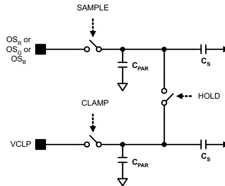
Figure 8. Sample and Hold Mode Simplified Input Diagram
