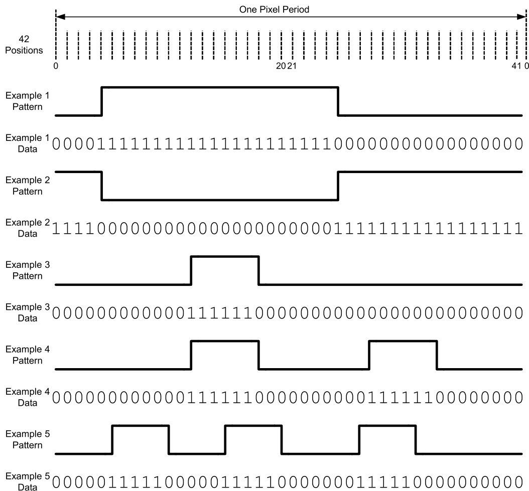
Figure 29. Pixel Timing - 42 Timing Points Per Pixel in Mode 3
