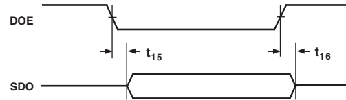
Figure 5. Serial Mode Timing for Data Output Enable and Serial Data Output ( T_{Sl} = \text{Logic Low} )
