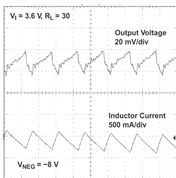
Figure 43. V_{NEG} in Continuous Current Mode
