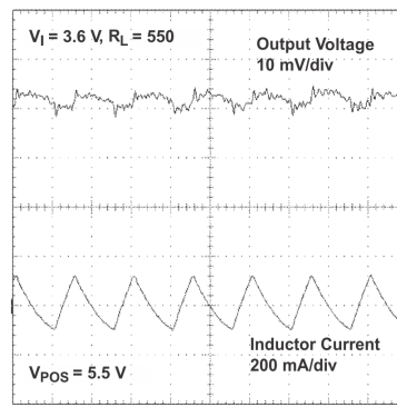
Figure 44. V_{POS} at Power-Save Mode Disabled
