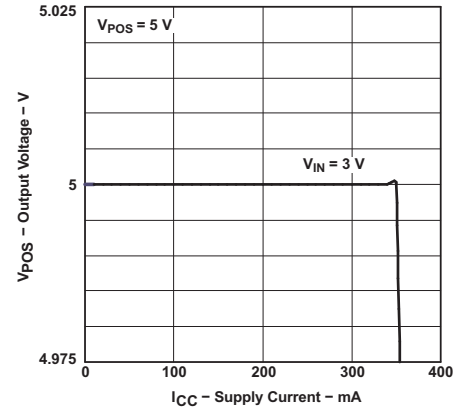
Figure 30. TPS65130 Output Voltage vs Output Current
