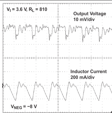
Figure 45. V_{NEG} at Power-Save Mode Disabled
