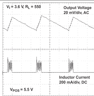
Figure 46. V_{POS} in Power-Save Mode
