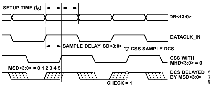
Figure 80. Setup Delay Measurement
