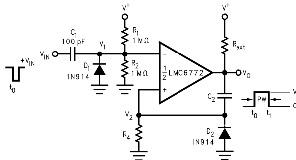
Figure 33. One-Shot Multivibrator
