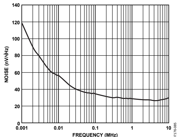
Figure 27. ADV3200 OSD Output Noise
