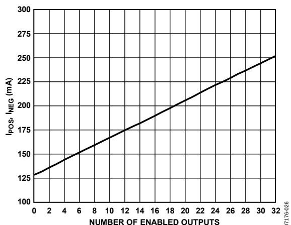
Figure 46. ADV3200 Supply Current vs. Enabled Outputs
