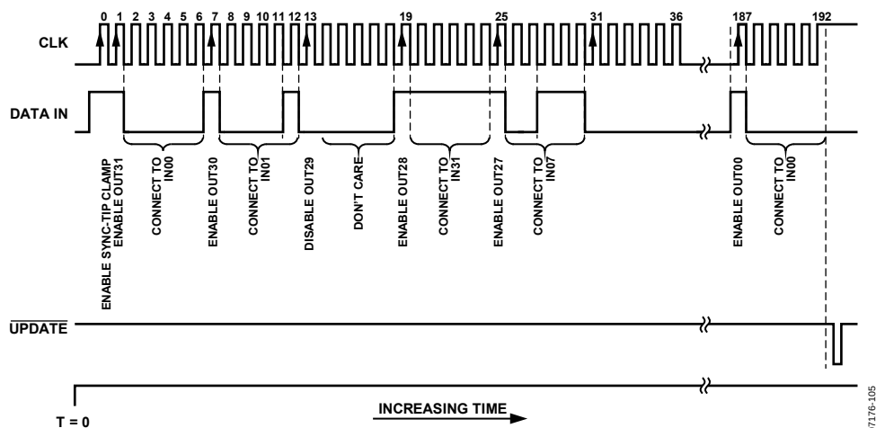
Figure 3. Programming Example
