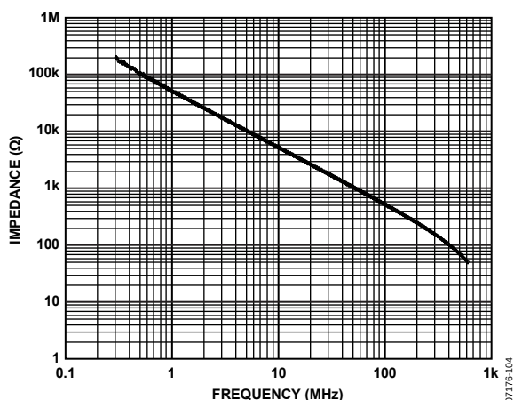
Figure 70. ADV3201 Input Impedance
