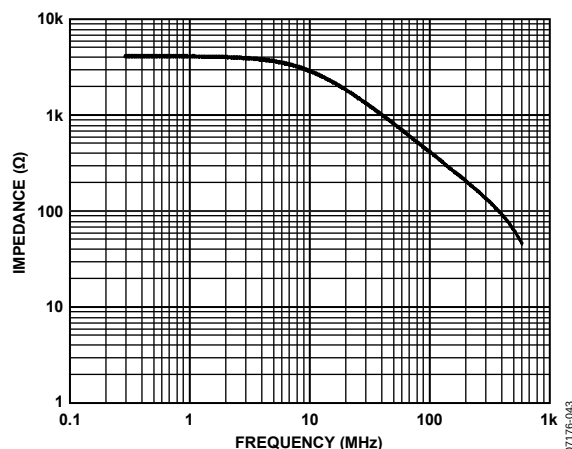
Figure 71. ADV3201 Output Impedance, Disabled
