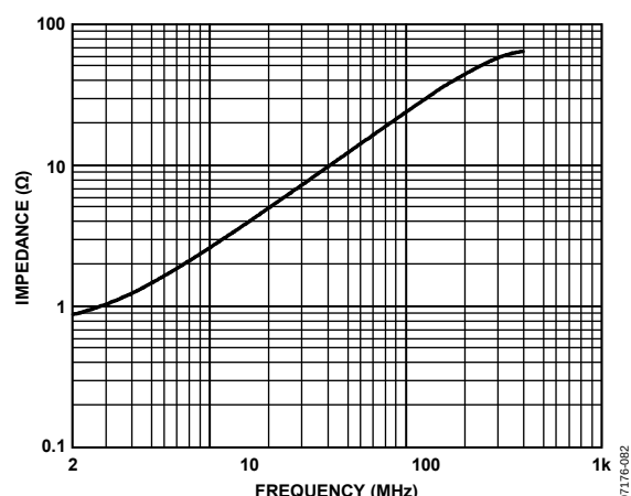
Figure 72. ADV3201 Output Impedance, Enabled
