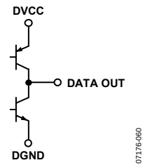
Figure 13. Logic Output (See Also Figure 16)
