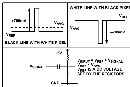
Figure 99. Pathological Case for Input Dynamic Range
