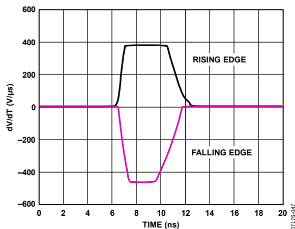
Figure 77. ADV3201 Slew Rate
