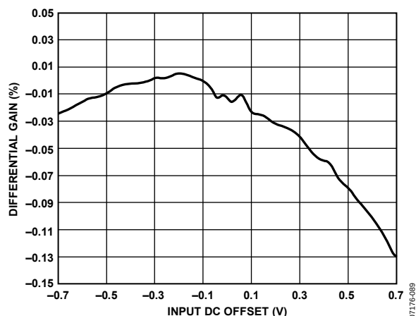
Figure 43. ADV3200 OSD Differential Gain, Carrier Frequency = 3.58 MHz, Subcarrier Amplitude = 300 mV p-p
