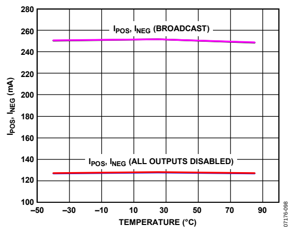
Figure 45. ADV3200 Supply Current vs. Temperature
