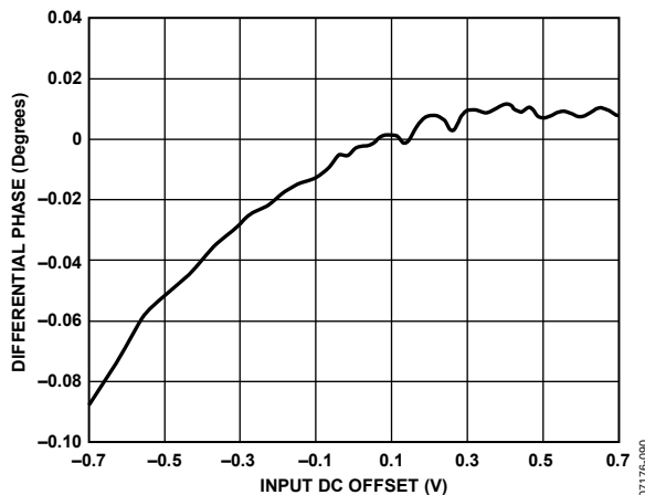
Figure 44. ADV3200 OSD Differential Phase, Carrier Frequency = 3.58 MHz, Subcarrier Amplitude = 300 mV p-p
