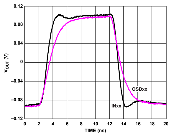
Figure 73. ADV3201 Small Signal Pulse Response, 200 mV p-p
