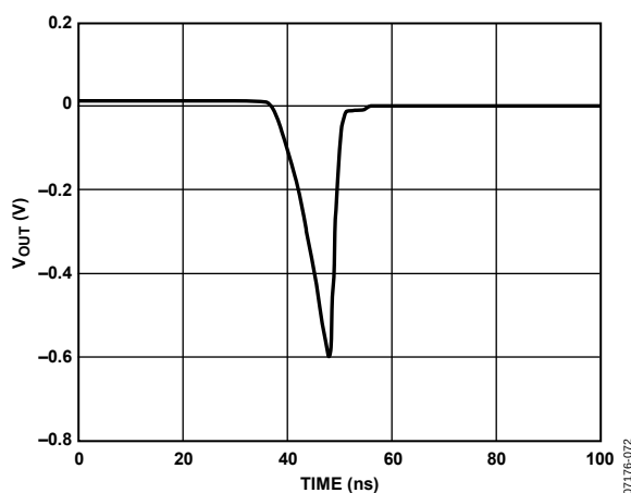
Figure 78. ADV3201 Switching Glitch
