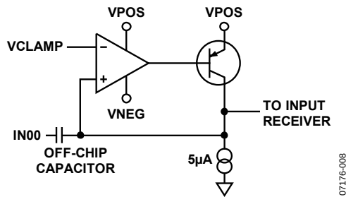
Figure 98. Conceptual Diagram of Sync-Tip Clamp in an AC-Coupled Application
