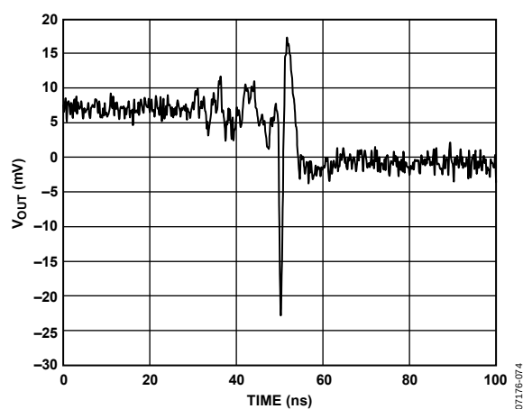
Figure 79. ADV3201 OSD Switching Glitch
