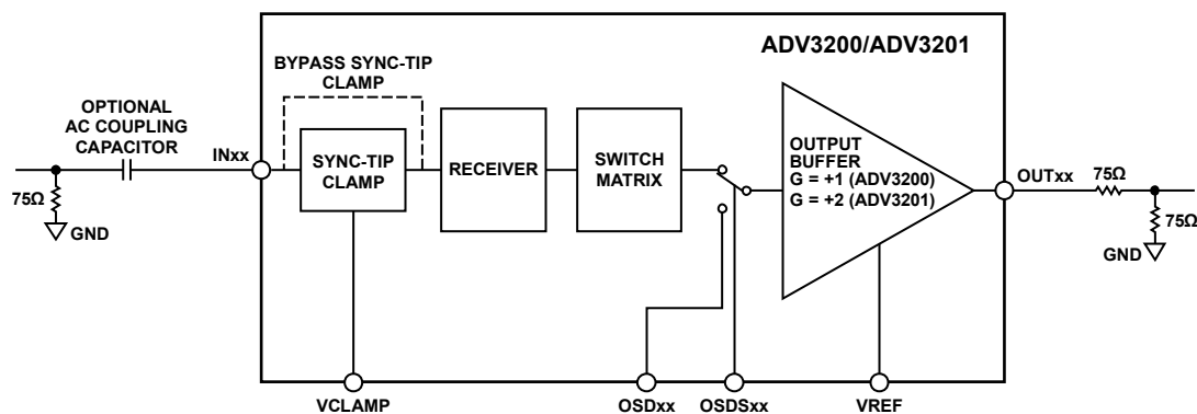
Figure 97. ADV3200/ADV3201 Signal Chain (Single I/O Path)
