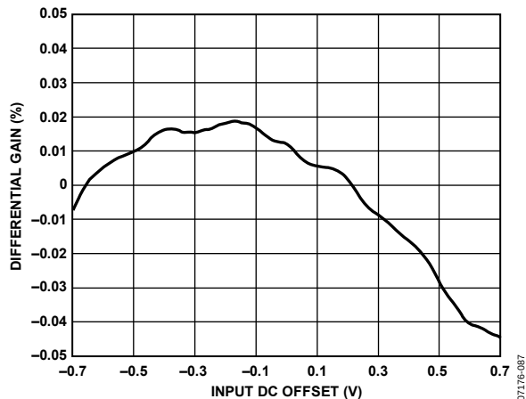
Figure 41. ADV3200 Differential Gain, Carrier Frequency = 3.58 MHz, Subcarrier Amplitude = 300 mV p-p
