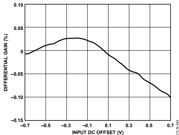
Figure 80. ADV3201 Differential Gain, Carrier Frequency = 3.58 MHz, Subcarrier Amplitude = 300 mV p-p
