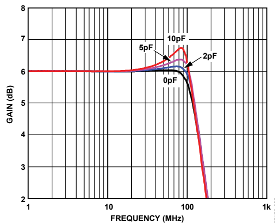
Figure 59. ADV3201 Large Signal Frequency Response with Capacitive Loads, 2 V p-p
