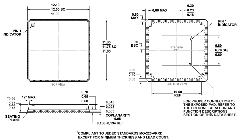
Figure 49. 88-Lead Lead Frame Chip Scale Package [LFCSP_VQ] 12 mm × 12 mm Body, Very Thin Quad (CP-88-5) Dimensions shown in millimeters
