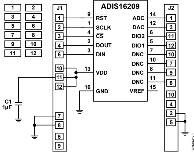
Figure 30. Electrical Schematic
