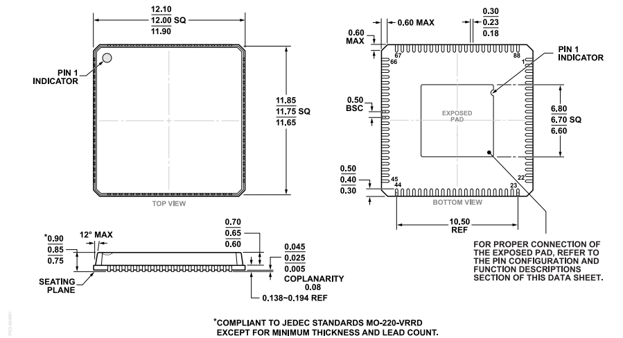
Figure 50. 88-Lead Lead Frame Chip Scale Package [LFCSP_VQ] 12 mm × 12 mm Body, Very Thin Quad (CP-88-5) Dimensions shown in millimeters
