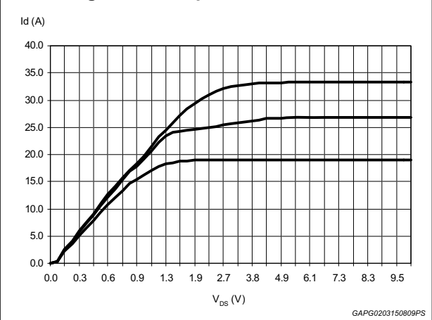
Figure 23. Output characteristics
