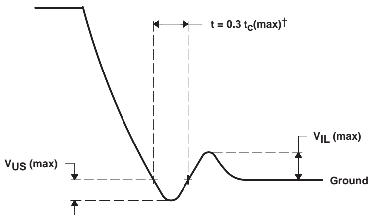
Figure 6–5. AC Transient Specification Fall Time
