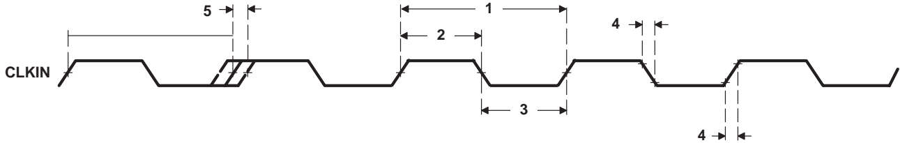
Figure 7–1. CLKIN Timing
