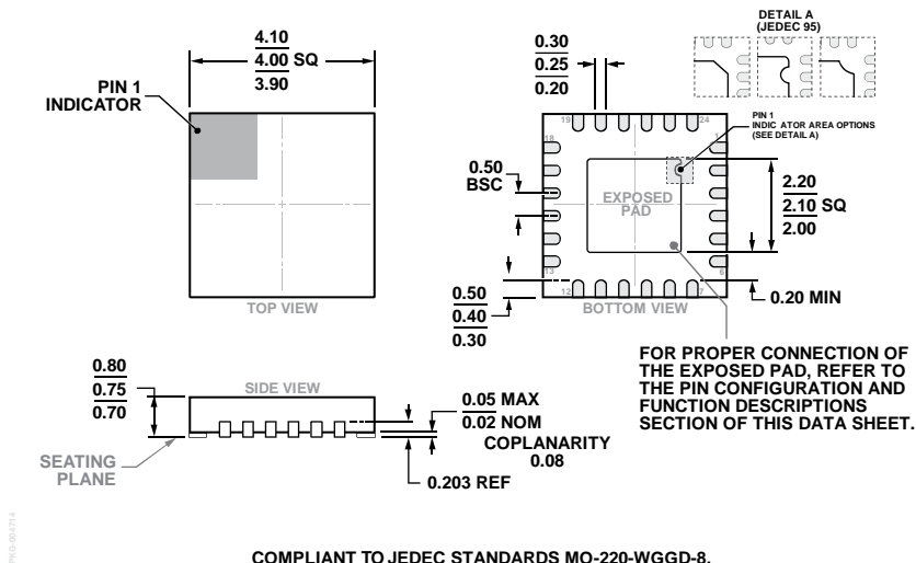
Figure 43. 24-Lead Lead Frame Chip Scale Package [LFCSP] 4 mm x 4 mm Body and 0.75 mm Package Height (CP-24-10) Dimensions shown in millimeters
