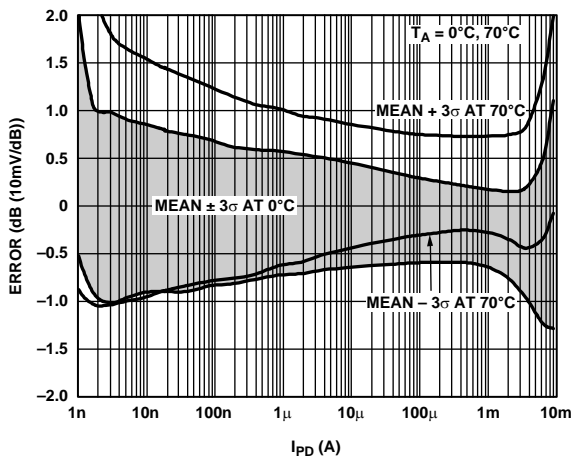
Figure 11. Law Conformance Error Distribution (3σ to Either Side of Mean)
