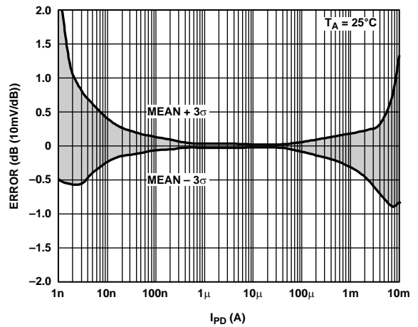
Figure 13. Law Conformance Error Distribution (3σ to Either Side of Mean)
