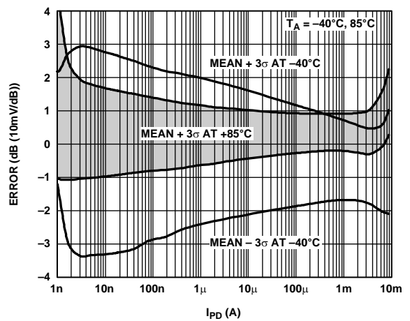
Figure 14. Law Conformance Error Distribution (3σ to Either Side of Mean)
