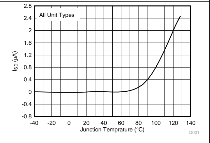
Figure 15. Disabled Supply Current ( I_{SD} ) vs Temperature
