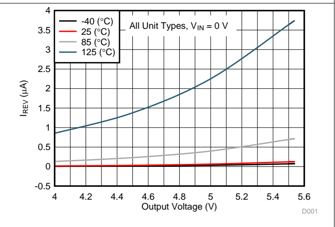
Figure 17. Reverse Leakage Current ( I_{REV} ) vs Output Voltage
