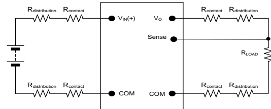
Figure 31. Remote sense circuit configuration
