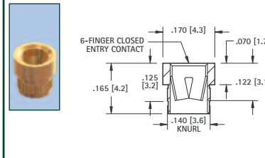
.084 (2.13) - .102 (2.6) PIN - PRESS-FIT
