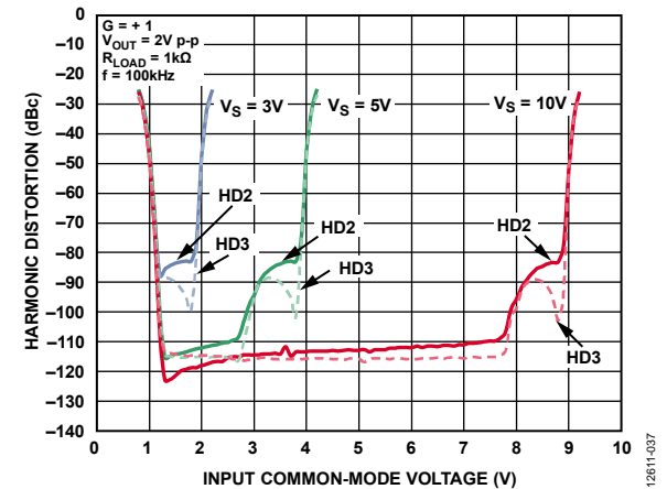
Figure 48. Harmonic Distortion vs. Input Common-Mode Voltage
