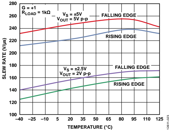
Figure 36. Slew Rate vs. Temperature
