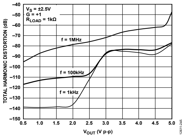
Figure 45. Total Harmonic Distortion vs. Output Voltage ( V_{out} )
