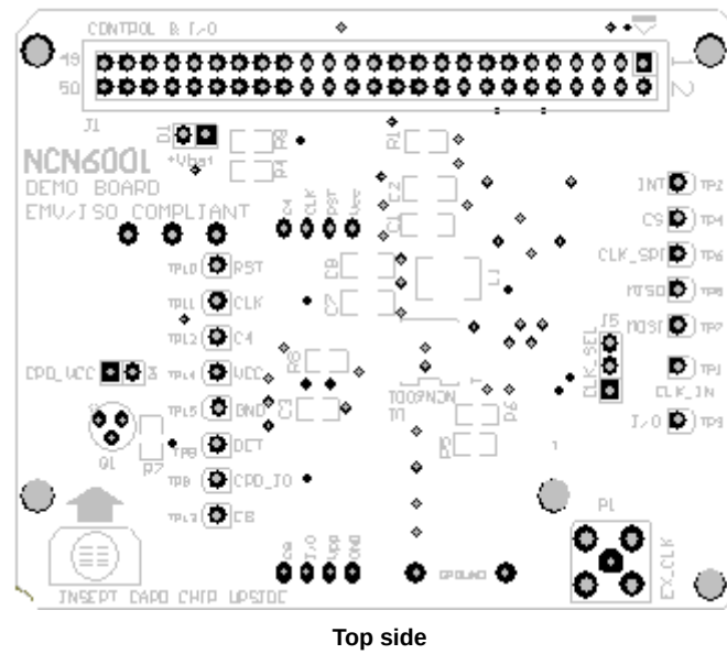
Figure 32. NCN6001 Demo Board Printed Circuit Board Layout
