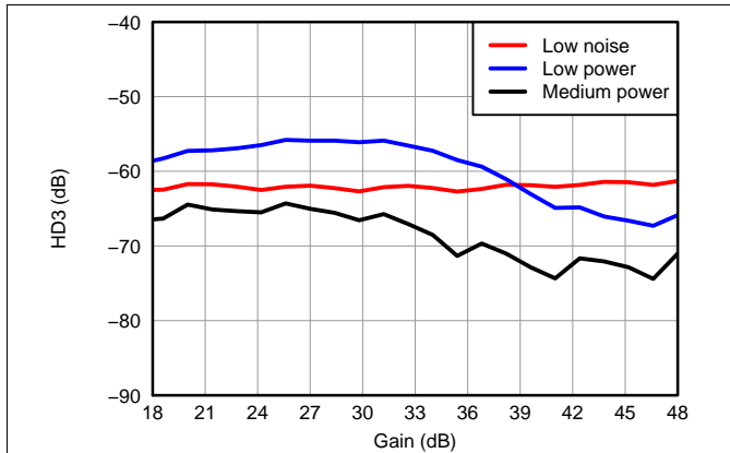
Figure 44. HD3 vs Gain, LNA = 24 dB and PGA = 24 dB and V_{OUT} = -1 dBFS
