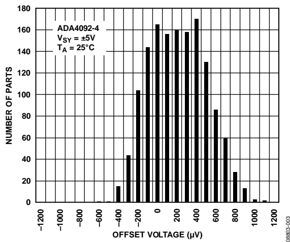
Figure 3. Input Offset Voltage Distribution, 10 V
