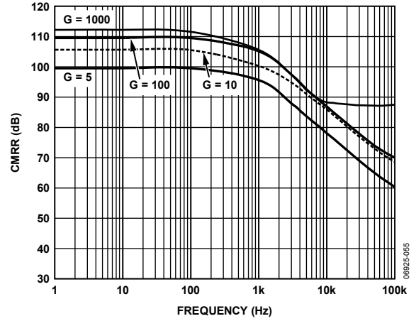
Figure 12. CMRR vs. Frequency, \pm V_S = \pm 12V
