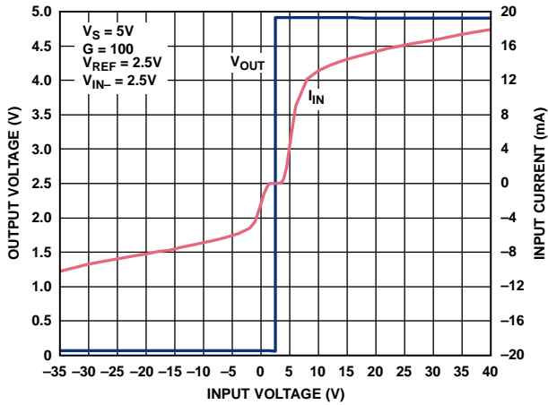
Figure 16. Input Overvoltage Performance; G = 100 , V_S = 5\text{ V}
