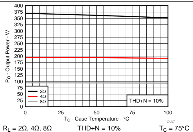
R_L = 2\Omega, 4\Omega, 8\Omega \text{THD+N} = 10\% T_C = 75^\circ\text{C} Figure 21. Output Power vs Case Temperature
