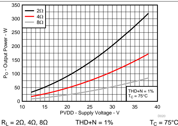
R_L = 2\Omega, 4\Omega, 8\Omega \text{THD+N} = 1\% T_C = 75^\circ\text{C} Figure 20. Output Power vs Supply Voltage
