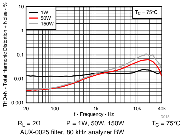
R_L = 2\Omega P = 1\text{W}, 50\text{W}, 150\text{W} T_C = 75^\circ\text{C} AUX-0025 filter, 80 kHz analyzer BW Figure 18. Total Harmonic Distortion+Noise vs Frequency
