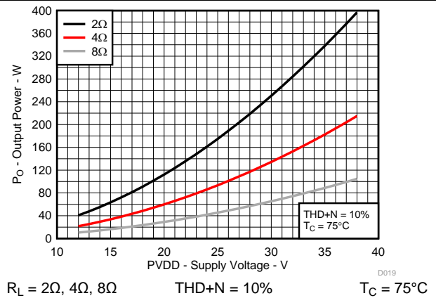
R_L = 2\Omega, 4\Omega, 8\Omega \text{THD+N} = 10\% T_C = 75^\circ\text{C} Figure 19. Output Power vs Supply Voltage
