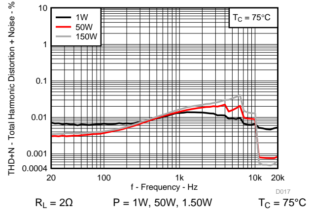
R_L = 2\Omega P = 1\text{W}, 50\text{W}, 150\text{W} T_C = 75^\circ\text{C} Figure 17. Total Harmonic Distortion+Noise vs Frequency
