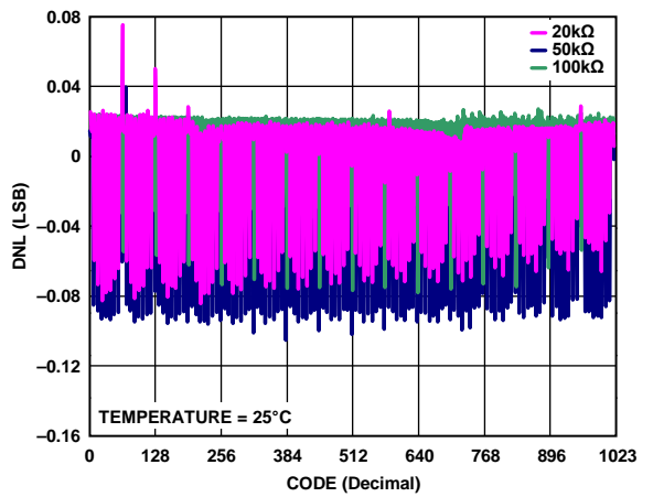
Figure 22. DNL in Normal Mode vs. Code vs. Nominal Resistance
