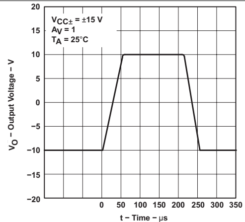
Figure 20. Voltage-Follower Large-Signal Pulse Response
