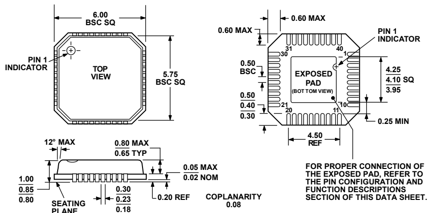
Figure 54. 40-Lead Lead Frame Chip Scale Package [LFCSP_VQ] 6 mm × 6 mm Body, Very Thin Quad (CP-40-1) Dimensions shown in millimeters
