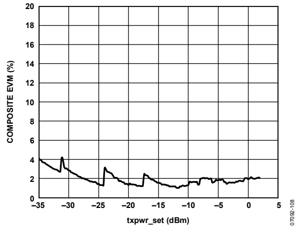
Figure 9. TXLBRF, UMTS Band V, Transmit EVM vs. txpwr_set (dBm), Four Calibration Points Applied, Transmit Frequency 881 MHz.
