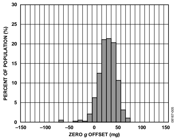
Figure 5. Y-Axis Zero g Offset at 25°C, V_S = 2.6 V
