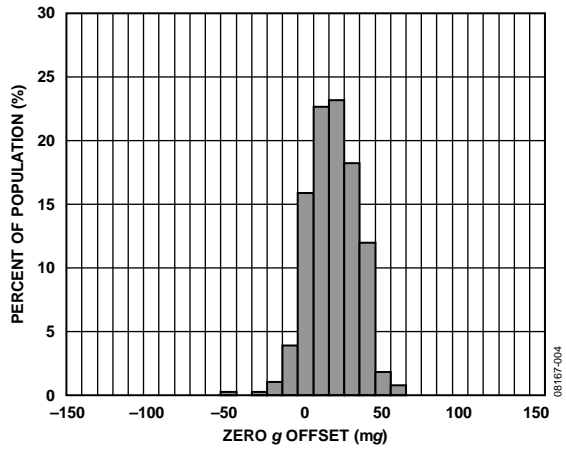
Figure 4. X-Axis Zero g Offset at 25°C, V_S = 2.6 V
