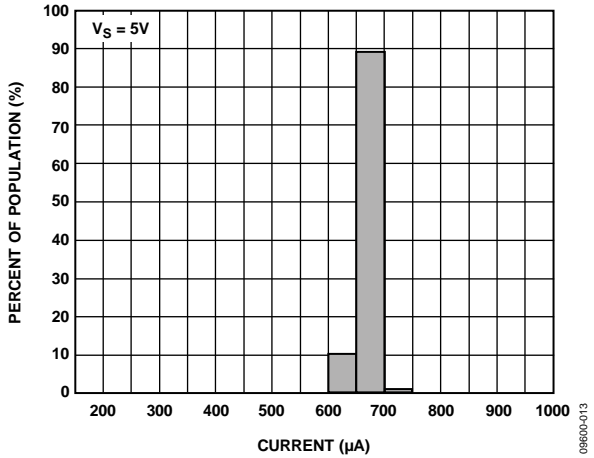
Figure 17. Supply Current at T_A = 25^\circ\text{C}
