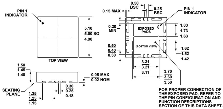
Figure 45. 16-Lead Lead Frame Chip Scale Package [LFCSP] 5 mm × 5 mm Body and 1.45 mm Package Height (CP-16-8) Dimensions shown in millimeters
