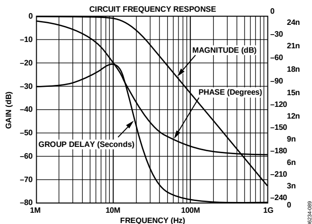
Figure 90. Output Filter Plot for SD, 16× Oversampling
