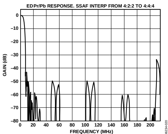
Figure 22. ED 8× Oversampling, Pr/Pb Filter (SSAF™) Response
