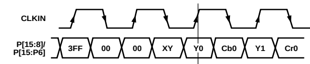
Figure 58. ED/HD-DDR Input Sequence (EAV/SAV)—Option B
