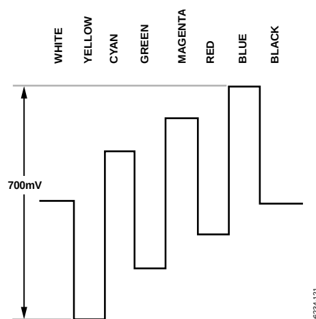
Figure 123. Pb Levels—PAL
