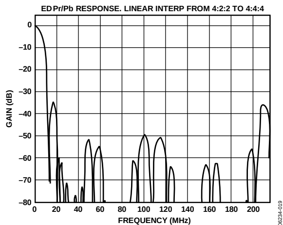
Figure 21. ED 8× Oversampling, Pr/Pb Filter (Linear) Response
