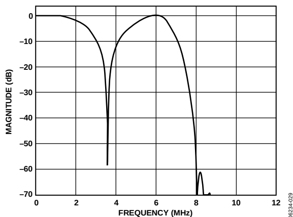
Figure 31. SD NTSC, Luma Notch Filter Response
