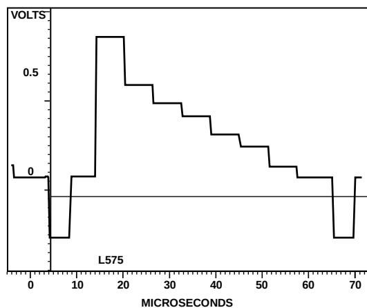
Figure 135. PAL Color Bars (75%)
