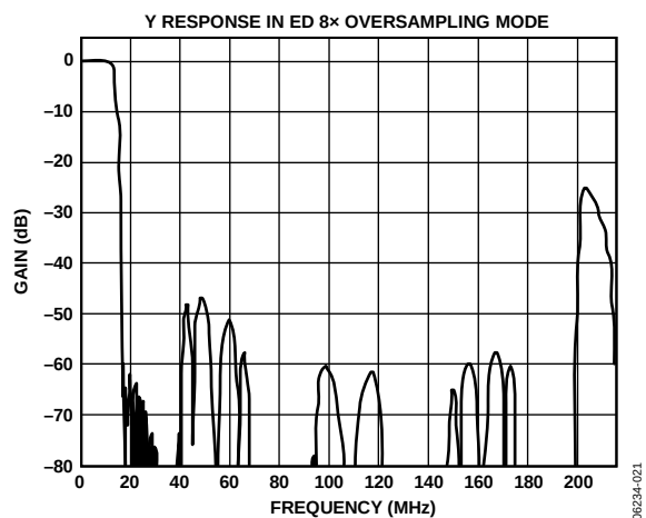
Figure 23. ED 8× Oversampling, Y Filter Response
