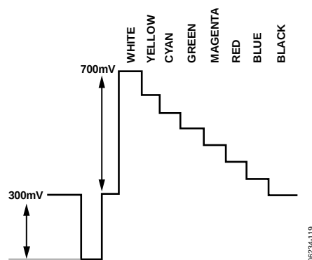
Figure 121. Y Levels—PAL
