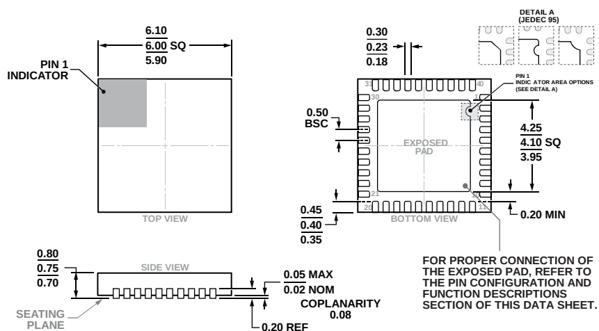
Figure 148. 40-Lead Lead Frame Chip Scale Package [LFCS] 6 mm × 6 mm Body and 0.75 mm Package Height (CP-40-9) Dimensions shown in millimeters
