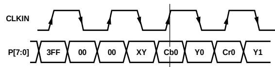
Figure 52. ED/HD-DDR Input Sequence (EAV/SAV)—Option A
