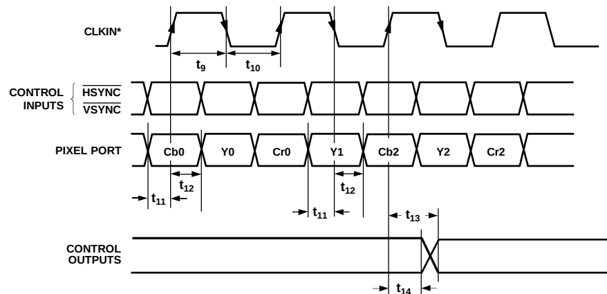
Figure 8. ED/HD-DDR Input, 8-/10-Bit 4:2:2 YCrCb ( \overline{\text{HSYNC}} / \overline{\text{VSYNC}} ), Input Mode 010
