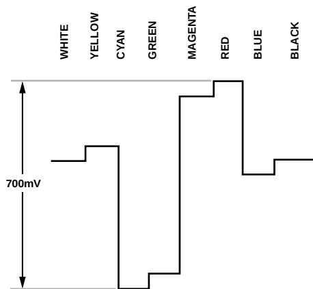
Figure 119. Pr Levels—NTSC
