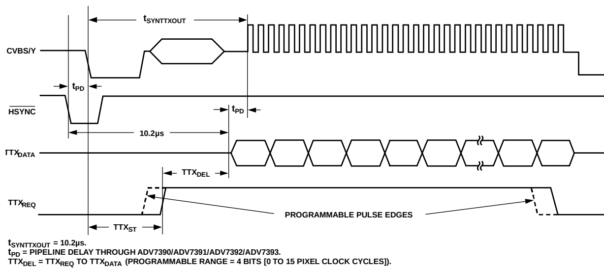
Figure 86. Teletext Functionality Diagram
