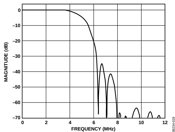
Figure 30. SD PAL, Luma Low-Pass Filter Response
