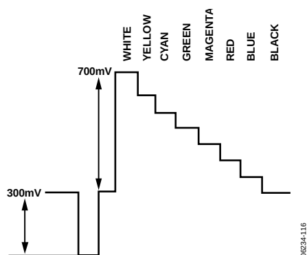
Figure 118. Y Levels—NTSC
