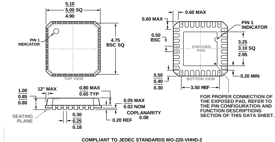
Figure 145. 32-Lead Lead Frame Chip Scale Package [LFCSP] 5 mm x 5 mm Body and 0.85 mm Package Height (CP-32-2)
