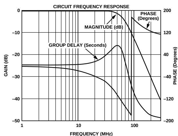
Figure 92. Output Filter Plot for HD, 4× Oversampling
