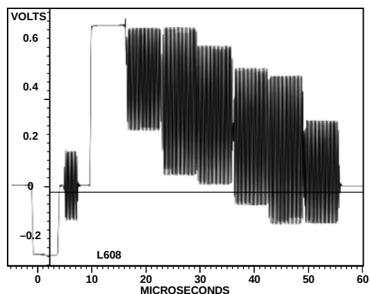
Figure 135. PAL Color Bars (75%)
