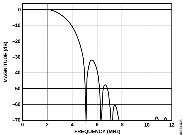
Figure 40. SD Chroma 3.0 MHz Low-Pass Filter Response
