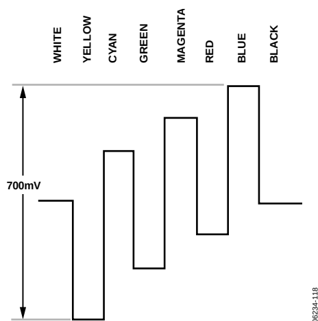
Figure 120. Pb Levels—NTSC
