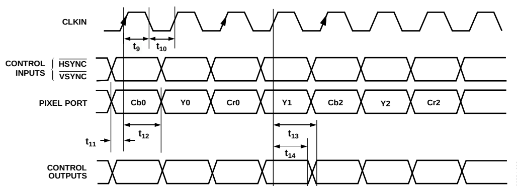
Figure 10. ED (at 54 MHz) Input, 8-/10-Bit 4:2:2 YCrCb (HSYNC/VSNC), Input Mode 111
