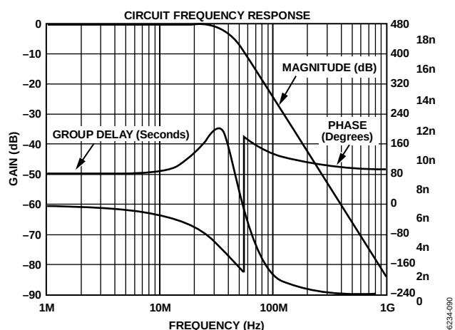
Figure 91. Output Filter Plot for ED, 8× Oversampling
