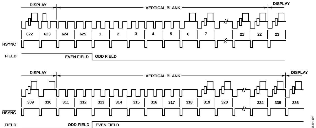
Figure 109. SD Timing Mode 1, Slave Option, PAL
