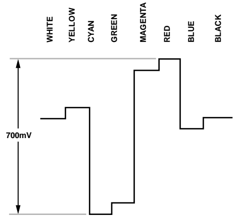
Figure 117. Pr Levels—PAL
