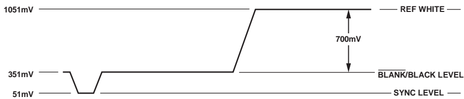
Figure 72. PAL RGB Video Levels
