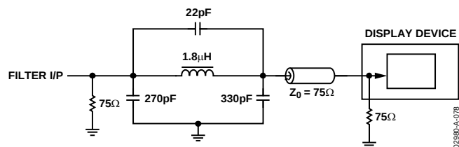
Figure 79. Output Filter
