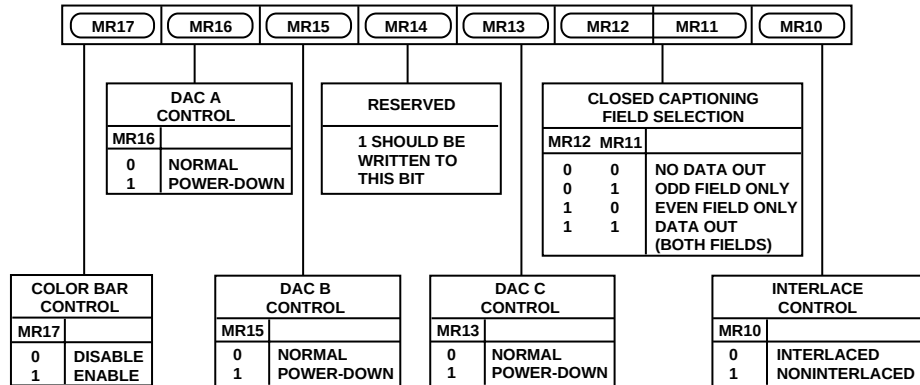
Figure 39. Mode Register 1
