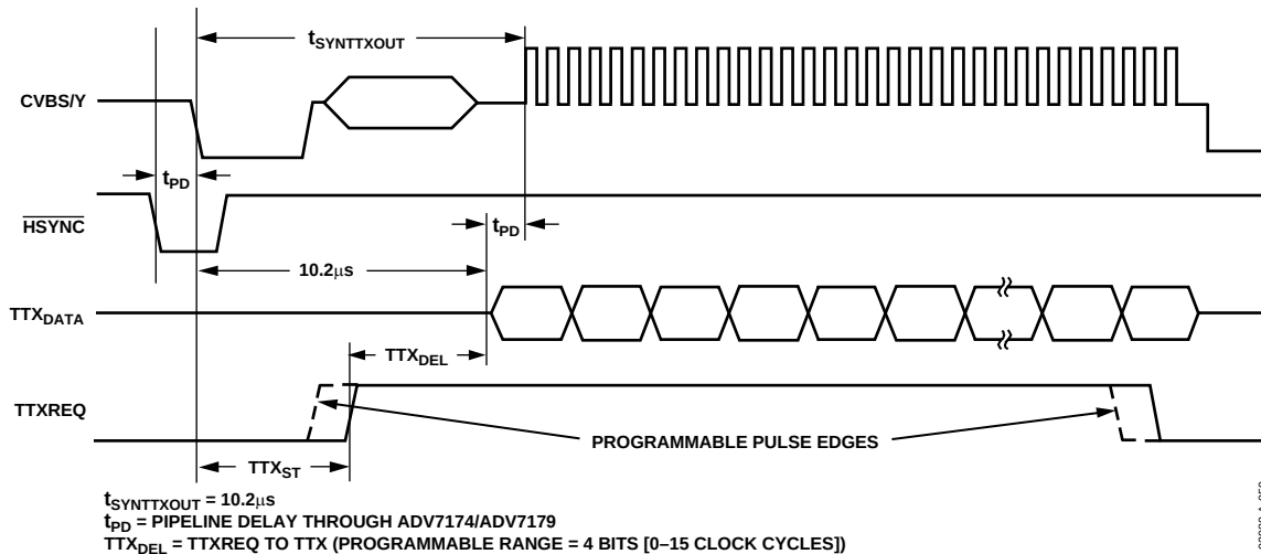
Figure 60. Teletext Functionality
