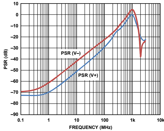
Figure 32. ADV3220 PSR
