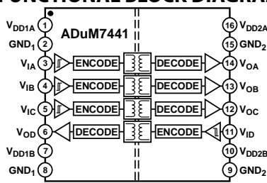
Figure 2. ADuM7441
