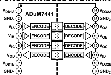
Figure 2. ADuM7441
