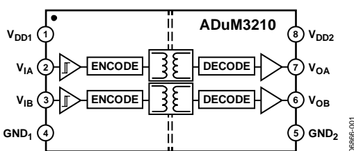
Figure 1. ADuM3210
